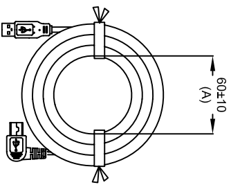
USB/A MALE TYPE
