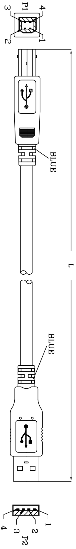
USB A/M MALE TYPE
