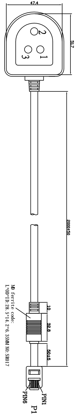
IT SOCKET
