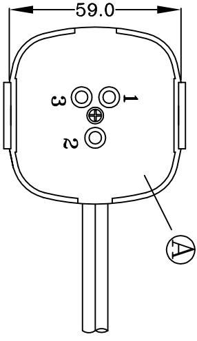
ITALIAN PLUG (P3)
